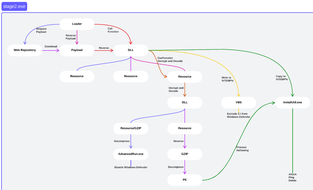
Figure 1: stage2.exe Execution Process Template
